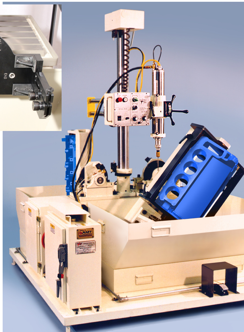
Combined AC Block and Head Machine with motorized height and indexed rotatable work holders
