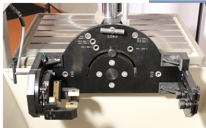
Shot-Pin Indexing for rotatable work holders
